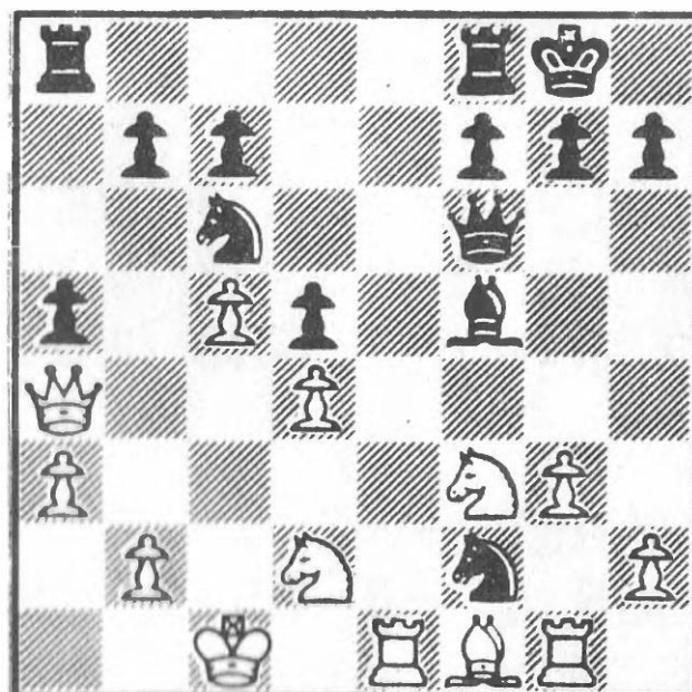
55 After 15 a3
